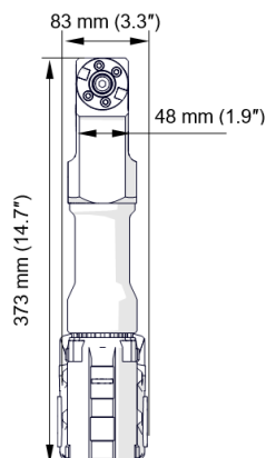
PRO-2 PB with battery drive
