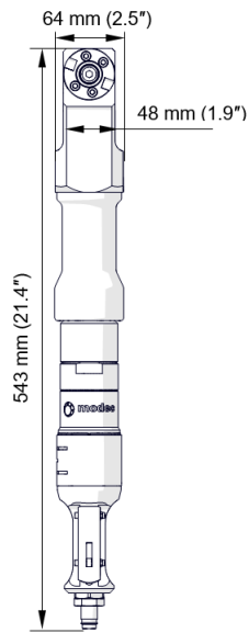
PRO-2 PB with pneumatic motor
